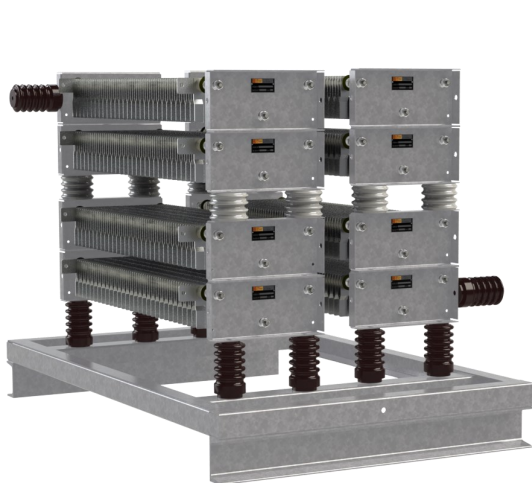
IP00 resistor: 14 Ohm. 500 Amp. -10 sec Insulation level: 12 kV.
